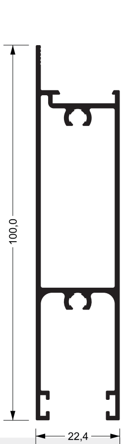
SU-225 1,005 kg/m
