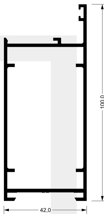
P-268 1,362 kg/m
