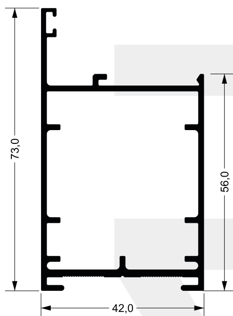
P-250 1,166 kg/m
