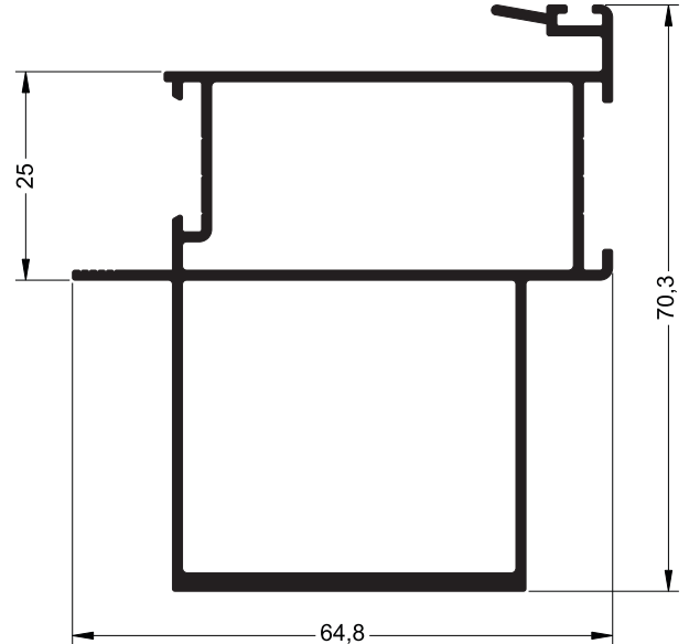
SU-290 1,066 kg/m
