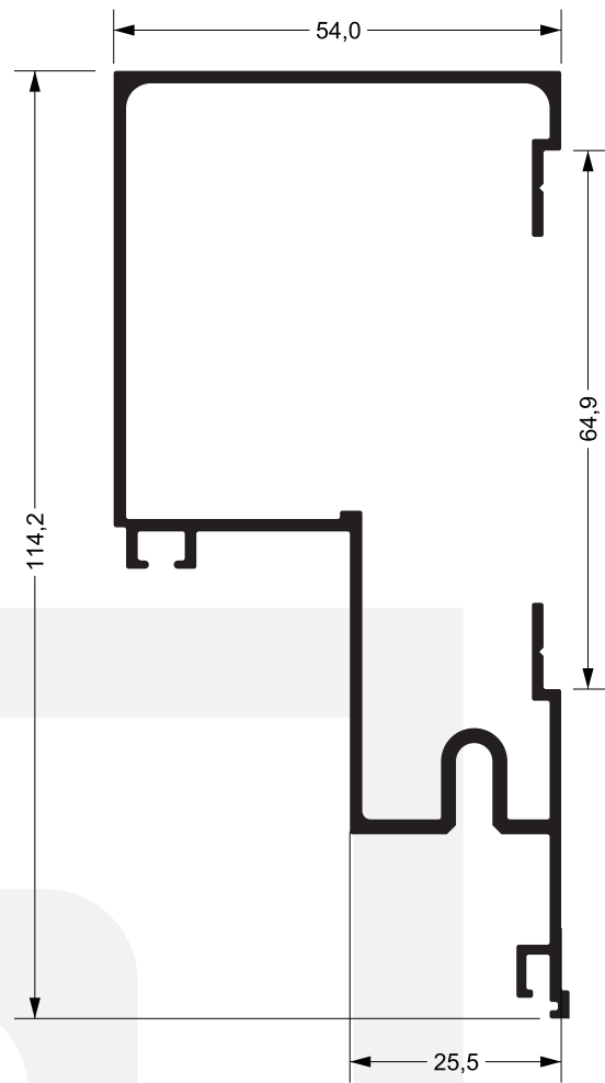
RA-235 1,544 kg/m
