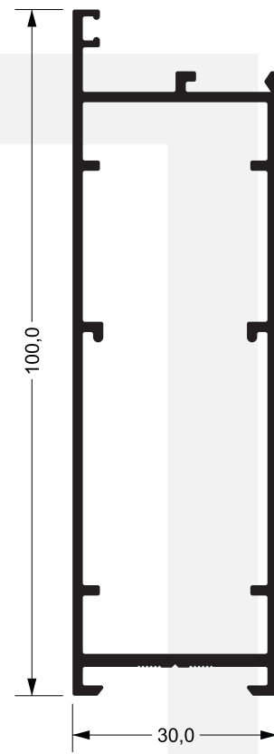
P-264 1,122 kg/m
