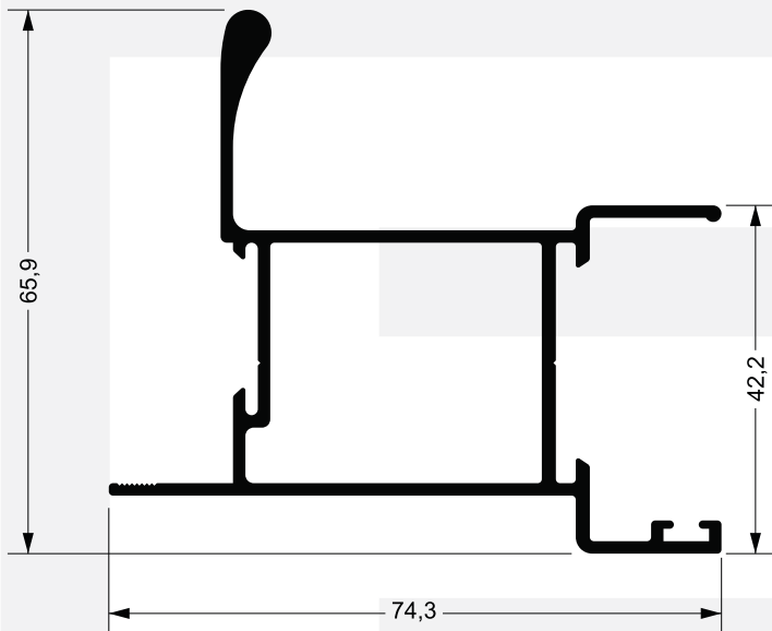
LG-020 1,119 kg/m
