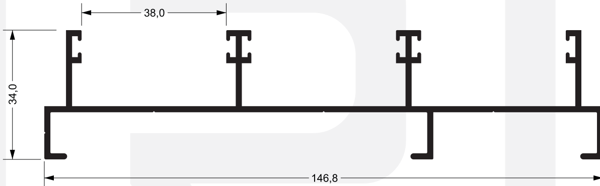
LG-064 1,282 kg/m
